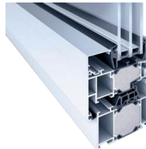
W 72 Construction depth 72 mm. Modular system with highly flexible design capabilities. Enhanced anti-security enabling classification up to RC3 standard.
