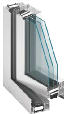
MB 86 Aero Construction depth of 77 mm.
