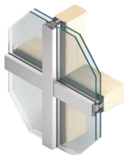
MB-SR 50 A Timber-aluminum curtain walls.
