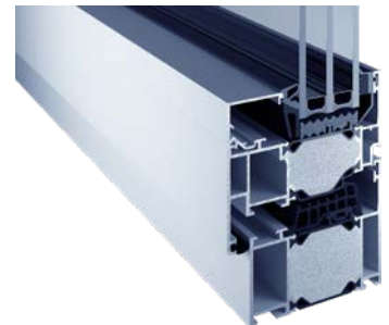
MB Slide System MB-SLIDE is designed for the manufacture of thermally insulated doors and sliding windows.
