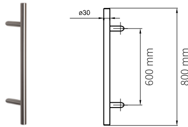
External pull bar – straight with 45° mounting (stainless steel), length 800 mm
