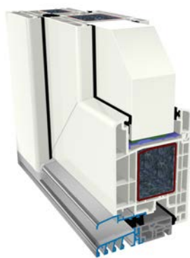
KOMBISYSTEM Inserted panel Panel depth 44 mm
