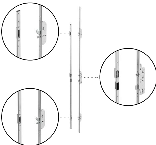
3 point espagnolette – with hooks
