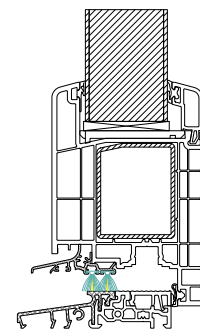
KOMBISYSTEM Inserted panel U_D from 0,86 W/m 2 K
