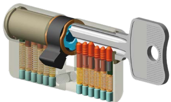
Class A cylinder
